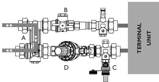
Flushing of main pipe line
